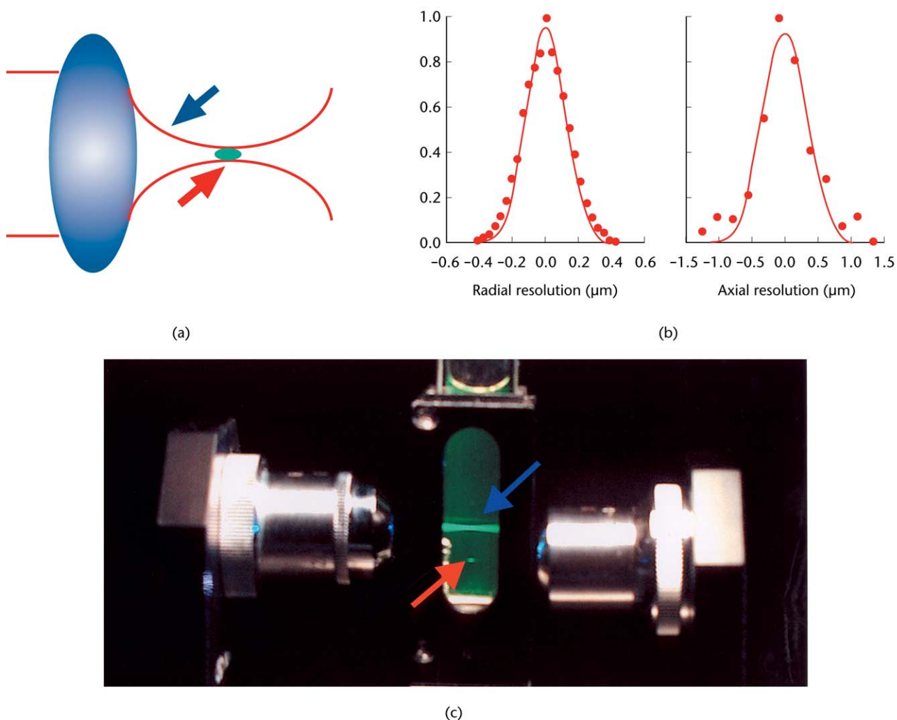
Figure 2 A schematic representation of the localisation of two-photon excitation. (a) Infrared light (blue arrow) is focused by an objective lens and fluorescence (red arrow) occurs only at the focal volume. (b) A detailed excitation profile of the two-photon excitation volume. The full width at half-maximum of the excitation profile is 0.3\ \mu\text{m} along the radial direction (left) and is 0.9\ \mu\text{m} along the longitudinal direction (right) at a laser wavelength of 960 nm. (c) A demonstration of the localisation of two-photon excitation volume. Fluorescein solution is excited by one-photon excitation (blue arrow) via a 0.1 numerical aperture objective; fluorescence excitation is observed throughout the path of the laser beam. For two-photon excitation using a second objective with the same numerical aperture (red arrow), fluorescence excitation occurs only from a 3D localised spot.
